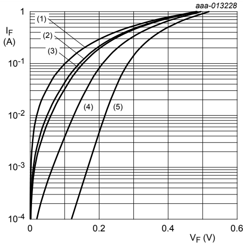
pulsed condition (1) T_j = 125\text{ }^\circ\text{C} (2) T_j = 85\text{ }^\circ\text{C} (3) T_j = 75\text{ }^\circ\text{C} (4) T_j = 25\text{ }^\circ\text{C} (5) T_j = -40\text{ }^\circ\text{C}
