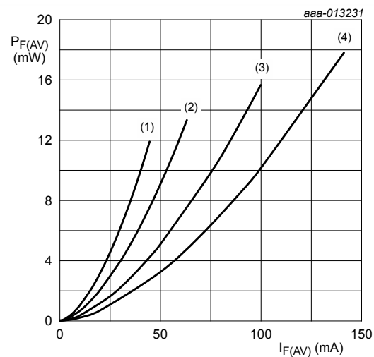
T_j = 125\text{ }^\circ\text{C} (1) \delta = 0.1 (2) \delta = 0.2 (3) \delta = 0.5 (4) \delta = 1
