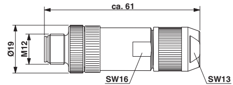
Dimensioned drawing
