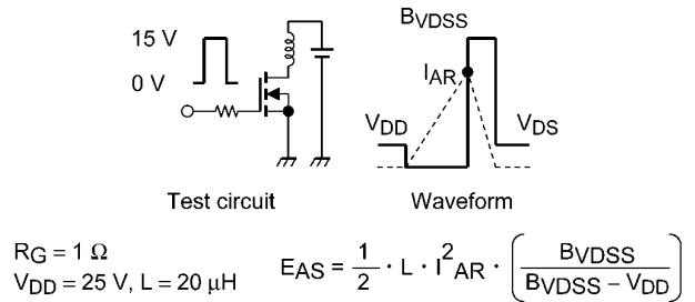
Fig. 8.15 Test Circuit/Waveform
