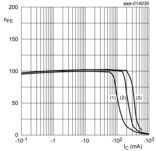
h_{FE} = f(I_C) T_{amb} = 25\text{ }^\circ\text{C} (1) V_{CE} = -10\text{ V} (2) V_{CE} = -25\text{ V} (3) V_{CE} = -50\text{ V}
