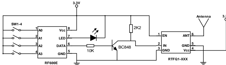
Transmitter Circuit
