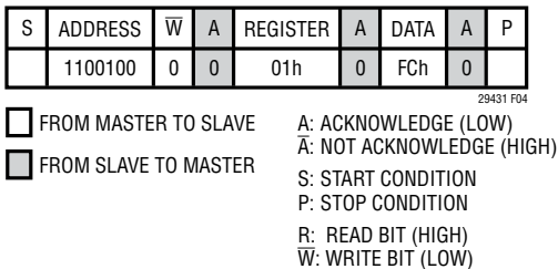
Figure 4. Writing FCh to the LTC2943-1 Control Register (B)
