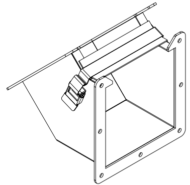
ISOMETRIV VIEW
