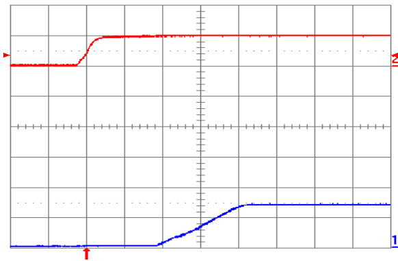
Fig. 1.0V.5: Turn-on transient for V_{out} = 1.0 V with application of V_{in} at full rated load current (resistive) and 100 \mu\text{F} external capacitance at V_{in} = 5 V. Top trace: V_{in} (5 V/div.); Bottom trace: output voltage (1 V/div.); Time scale: 2 ms/div.
