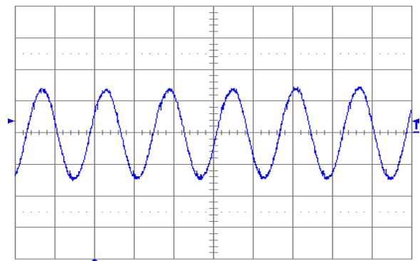
Fig. 1.8V.6: Output voltage ripple (20 mV/div.) at full rated load current into a resistive load with external capacitance 100\ \mu\text{F} ceramic + 1\ \mu\text{F} ceramic and V_{in} = 5\text{ V} for V_{out} = 1.8\text{ V} . Time scale: 2 \mu\text{s} /div.
