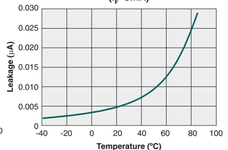
Typical Leakage vs. Temperature Measured Across Pins 4&6 ( I_F=5\text{mA} )
