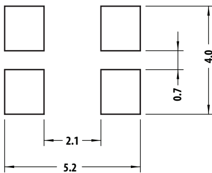
Figure 9. Recommended Soldering Land Pattern
