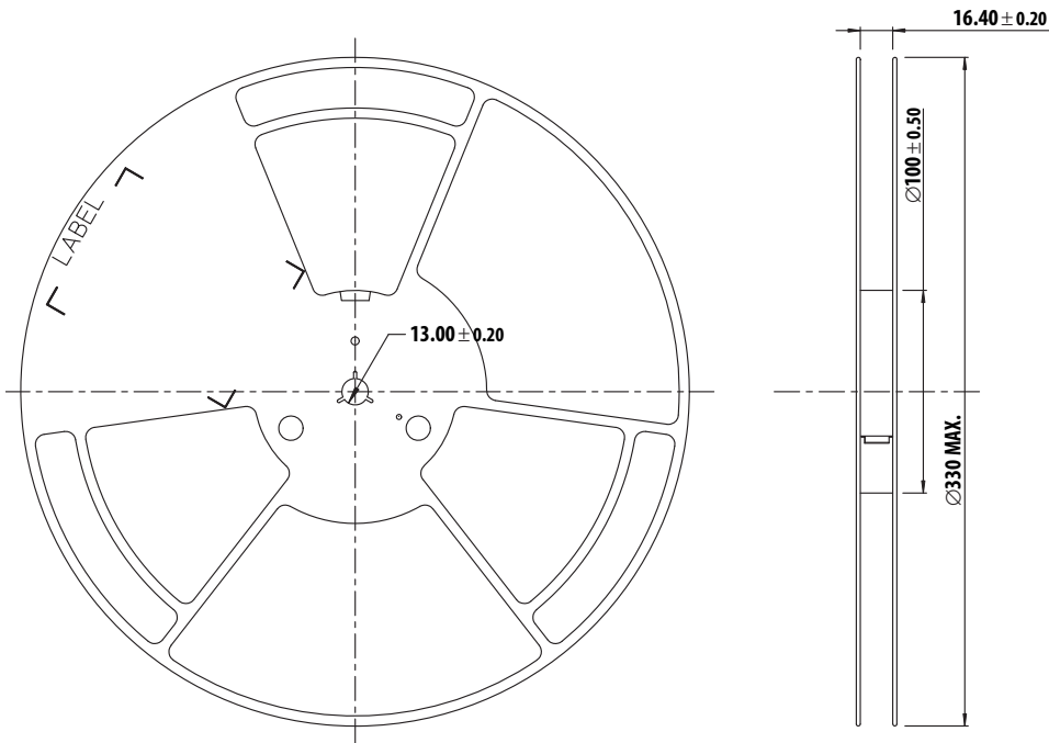
Figure 11. Reel Dimension
