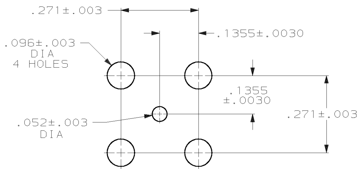
PCB CONFIGURATION
