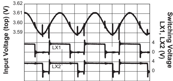
Time (0.2µs/div)
