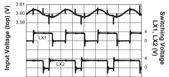
Time (0.2µs/div)
