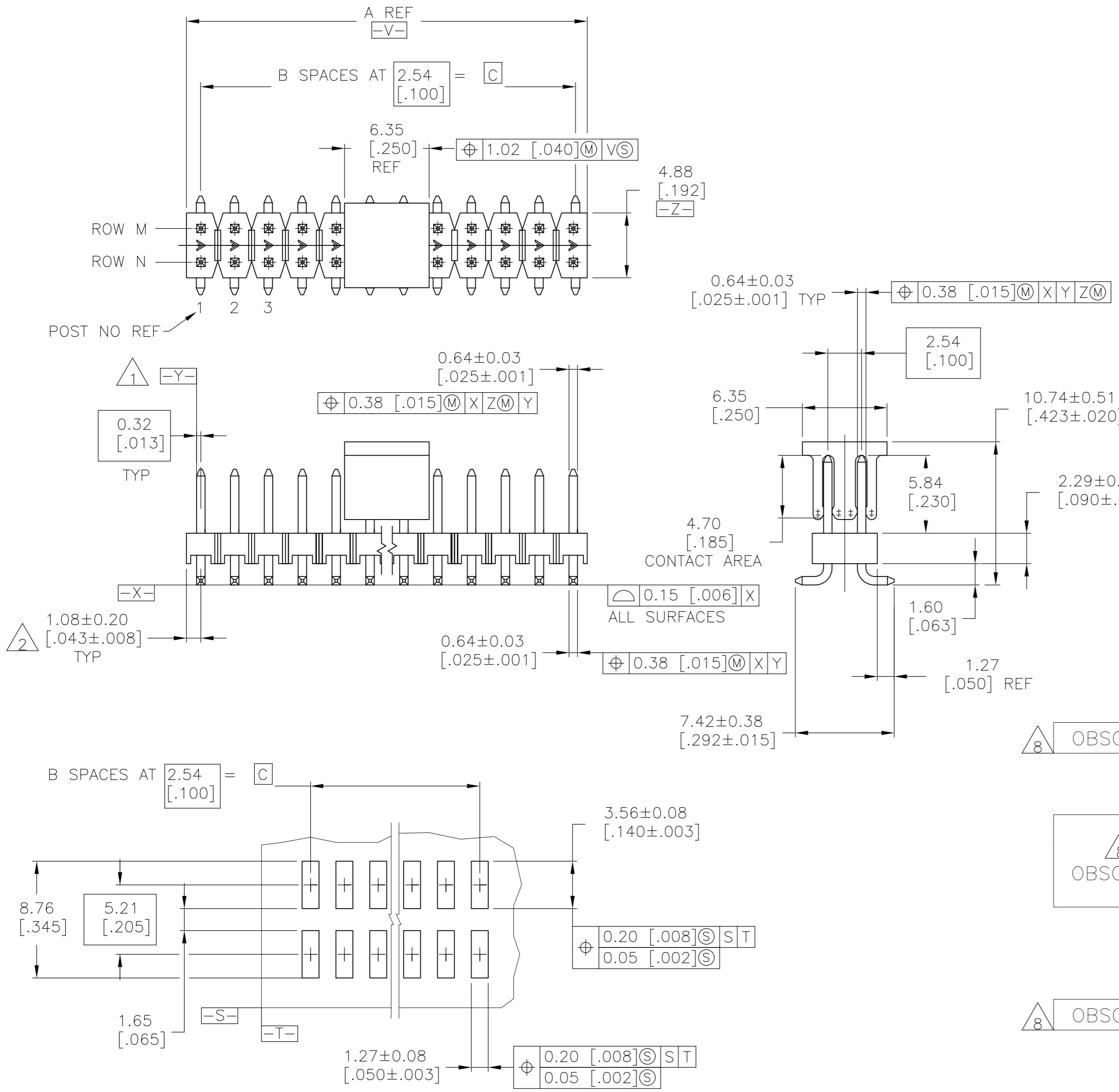
RECOMMENDED PCB LAYOUT FOR USE WITH 0.20 [.008] THICK STENCIL
