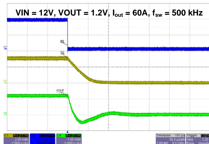
Fig. 6 Power Down Sequence (C3: EN, C1: SS1, C4: VOUT)
