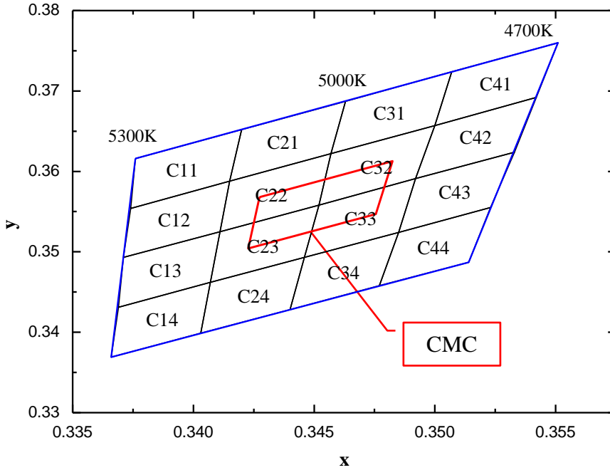
Fig 5-2. CIE Chromaticity Diagram
