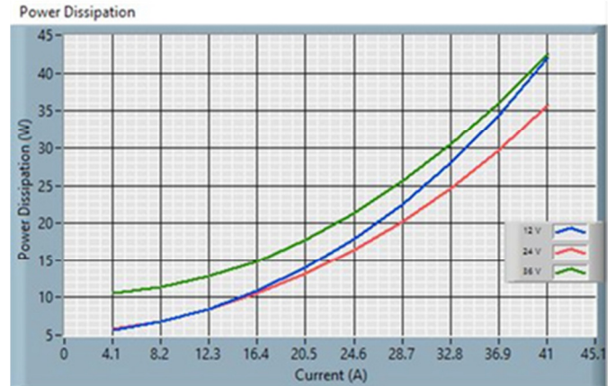
Fig. 5: ICH0141V1PC Power Dissipation
