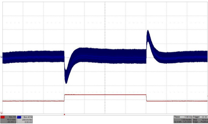
Fig. 30: Output voltage response to load current step change 50% - 75% - 50% (9A-13.5A-9A) with di/dt = 1A/μs at Vin = 24V. Top trace (C4): Output voltage (200 mV/div.). Bottom trace (C3): Load current (10A/div.). Co = 470μf/70mΩ. Time: 1ms/div.
