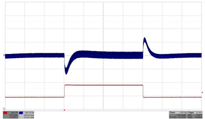
Fig. 31: Output voltage response to load current step change 50% - 100% - 50% (9A-18A-9A) with di/dt = 1A/μs at Vin = 24V. Top trace (C4): Output voltage (500 mV/div.). Bottom trace (C3): Load current (10A/div.). Co = 470μf/70mΩ. Time: 1ms/div.
