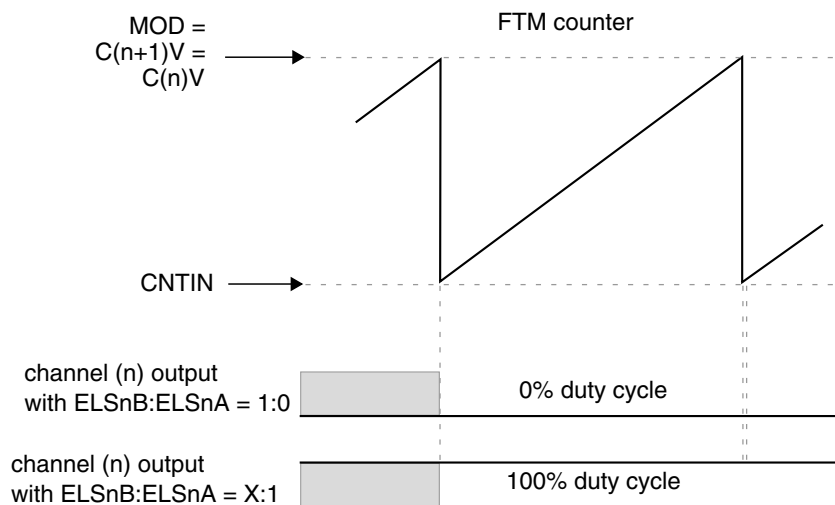
Figure 44-237. Channel (n) Output If (C(n)V = C(n+1)V = MOD)
