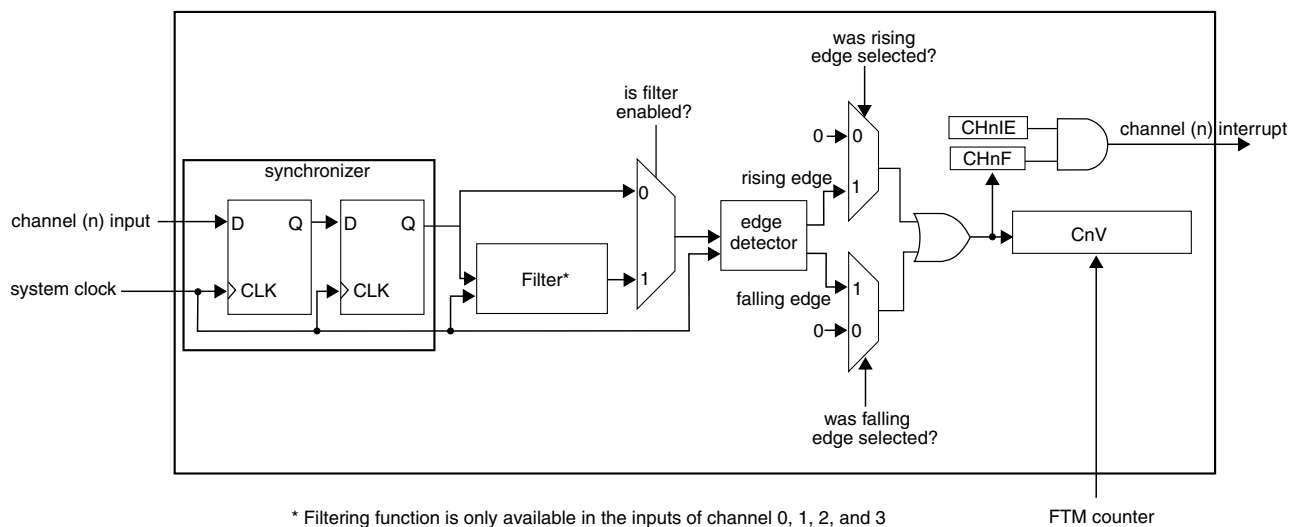
Figure 44-216. Input Capture Mode
