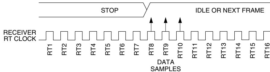
Figure 57-347. Fast data
