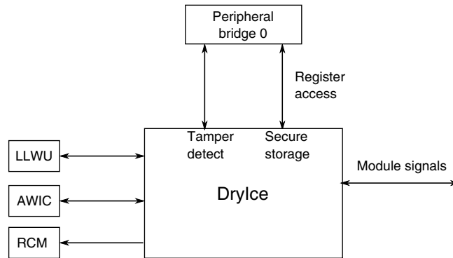
Figure 3-39. DryIce configuration
