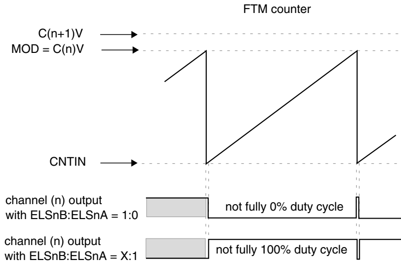
Figure 44-243. Channel (n) Output If (C(n+1)V > MOD) and (CNTIN < C(n)V = MOD)
