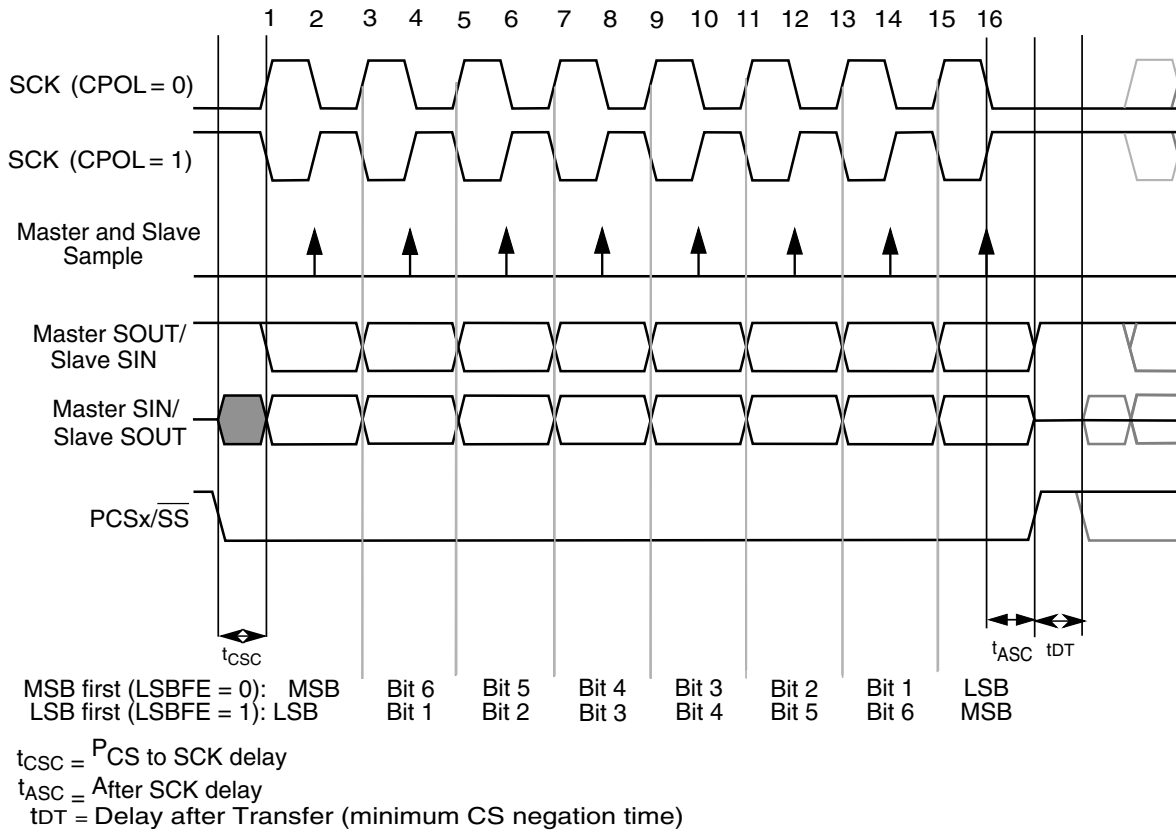
Figure 55-95. DSPI Transfer Timing Diagram (MTFE=0, CPHA=1, FMSZ=8)
