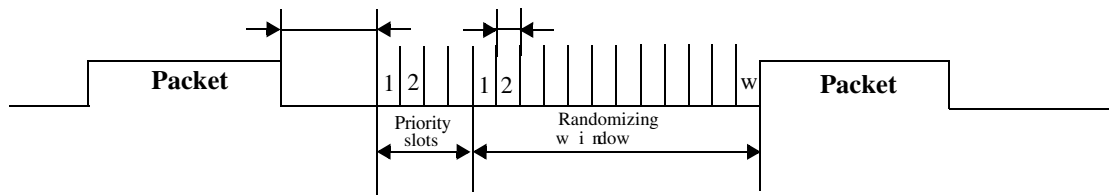
Figure 57-339. CEA709.1-B packet cycle
