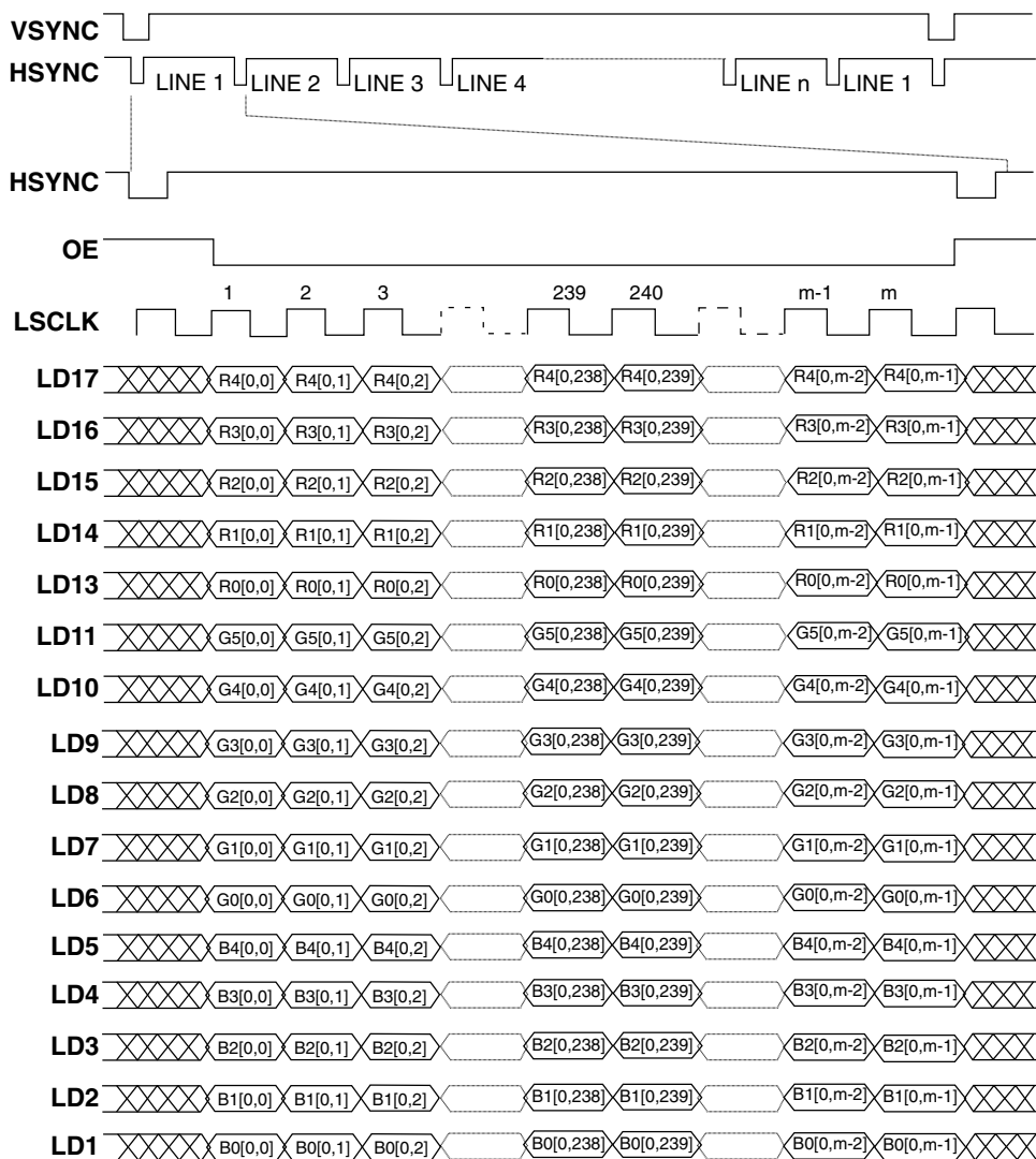
Figure 62-35. LCD Interface Timing for 16 bpp Active Matrix Color Panels
