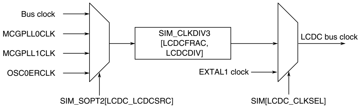
Figure 5-15. LCD controller clock generation
