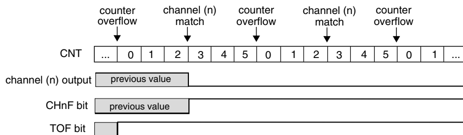
Figure 44-220. Example of the Output Compare Mode when the Match Clears the Channel Output
