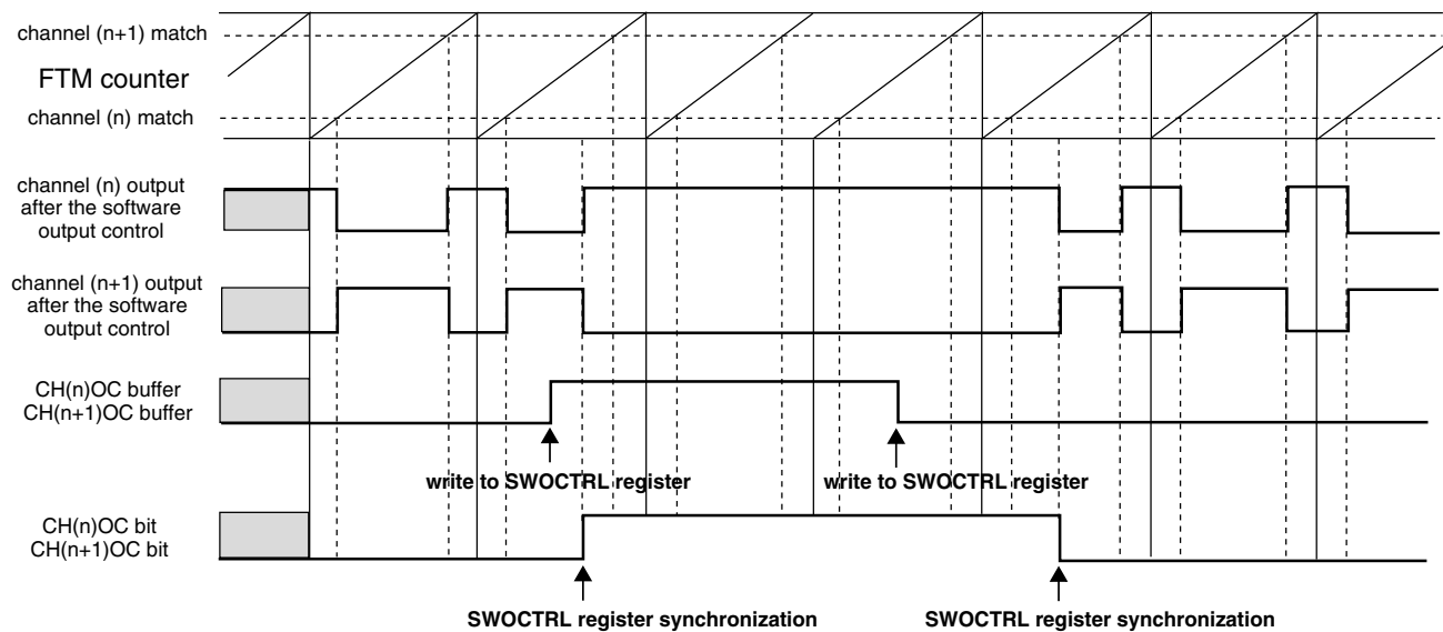
Figure 44-268. Example of Software Output Control in Combine and Complementary Mode
