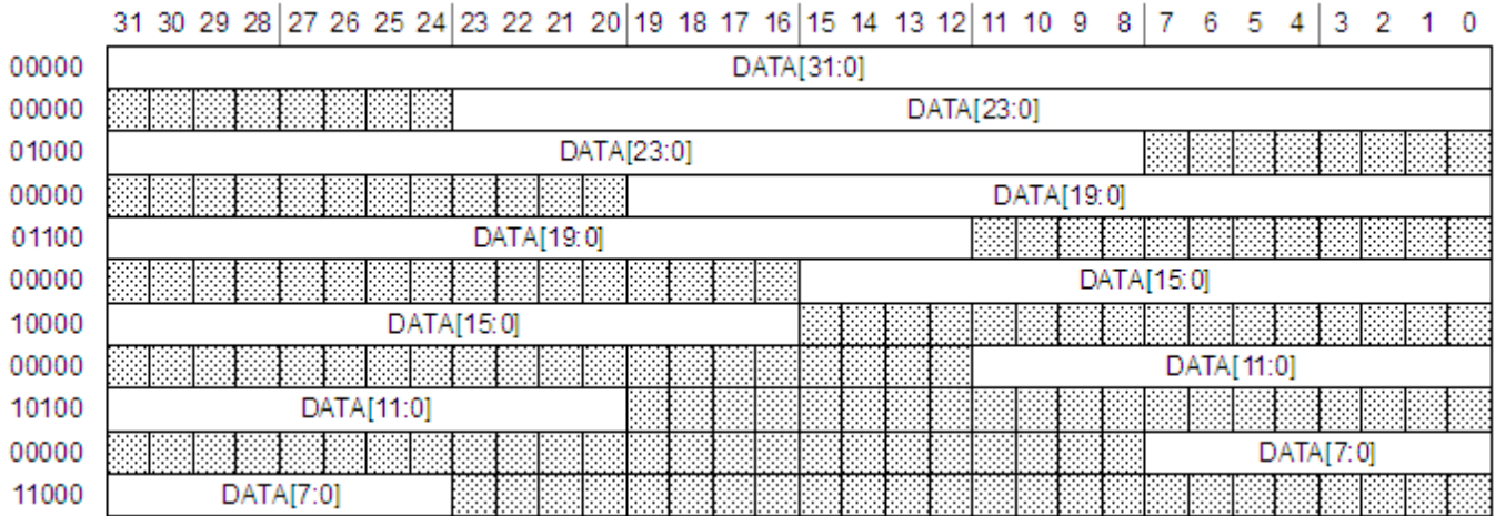
Figure 59-87. SAI First Bit Shifted, LSB First
