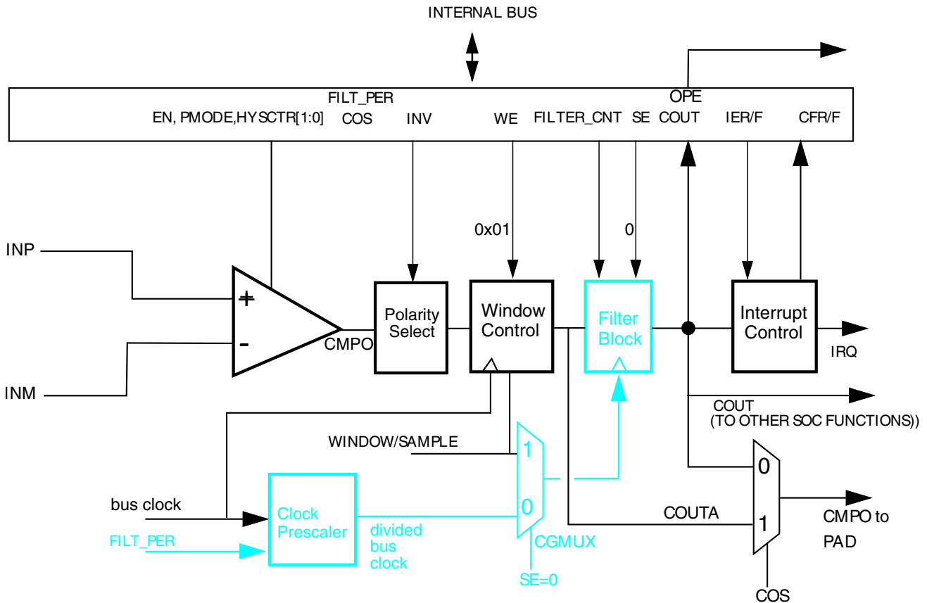
Figure 40-39. Windowed Mode
