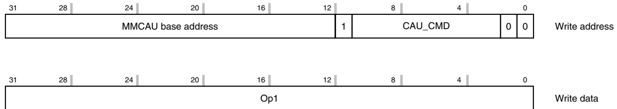
Figure 36-17. Indirect loads
