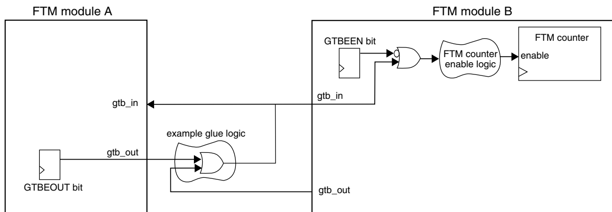
Figure 44-299. Global Time Base (GTB) Block Diagram
