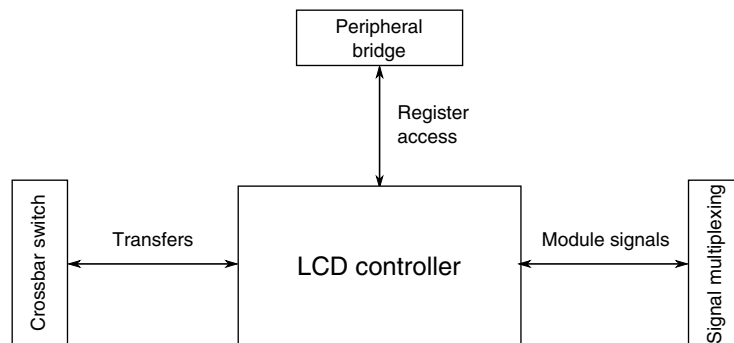
Figure 3-76. LCDC configuration
