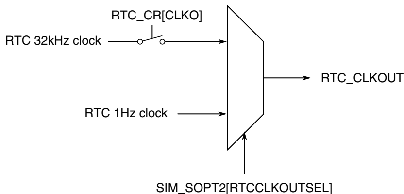
Figure 3-57. RTC_CLKOUT generation
