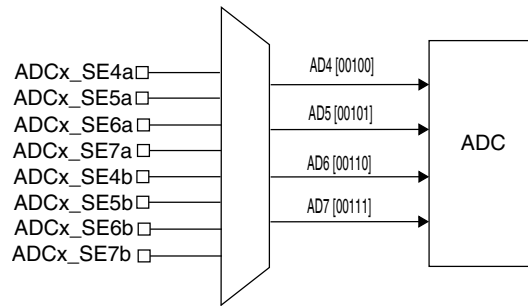
Figure 3-41. ADCx_SEn channels a and b selection
