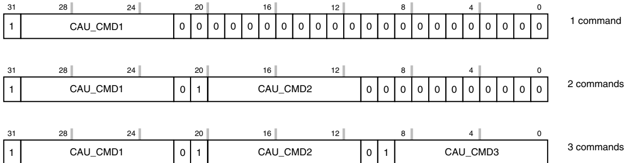
Figure 36-16. Direct loads
