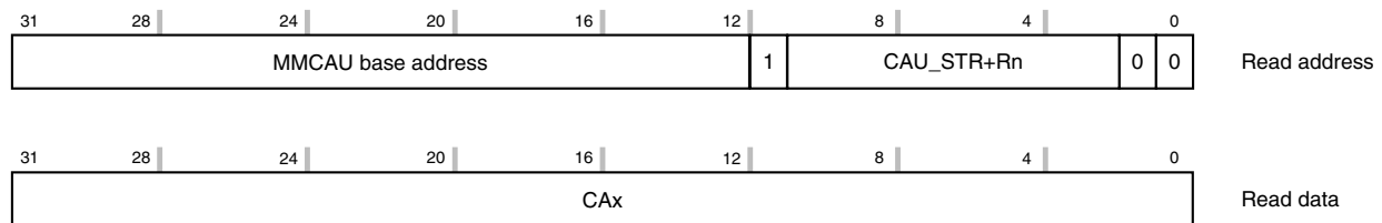
Figure 36-18. Indirect store
