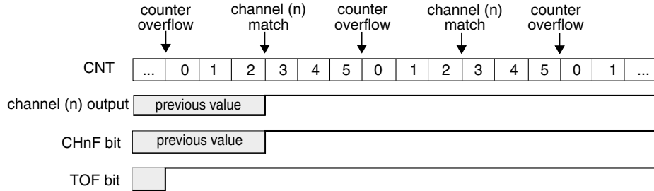
Figure 44-221. Example of the Output Compare Mode when the Match Sets the Channel Output
