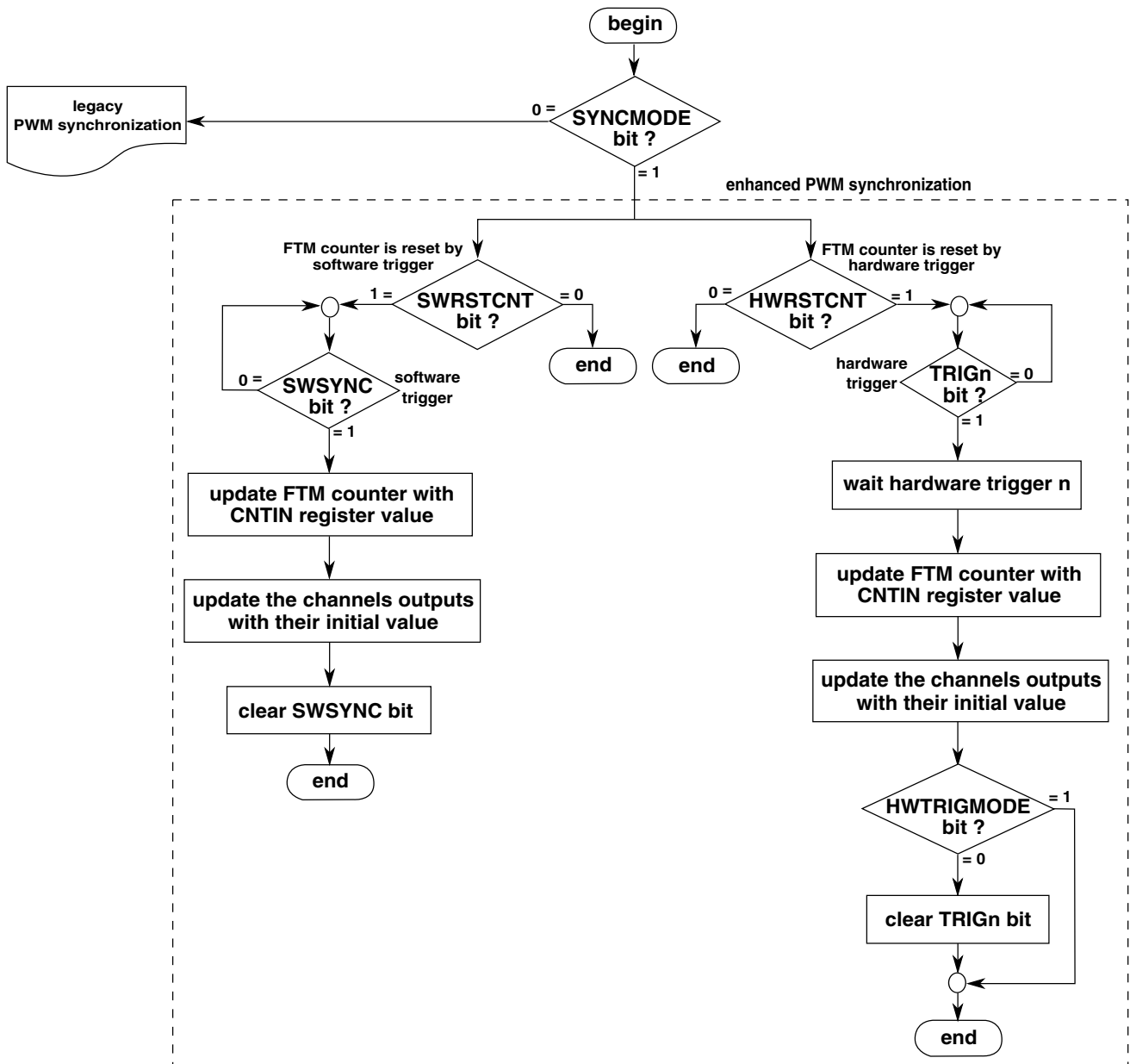
Figure 44-262. FTM Counter Synchronization Flowchart
