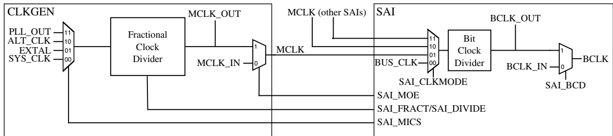
Figure 59-86. SAI Master Clock Generation
