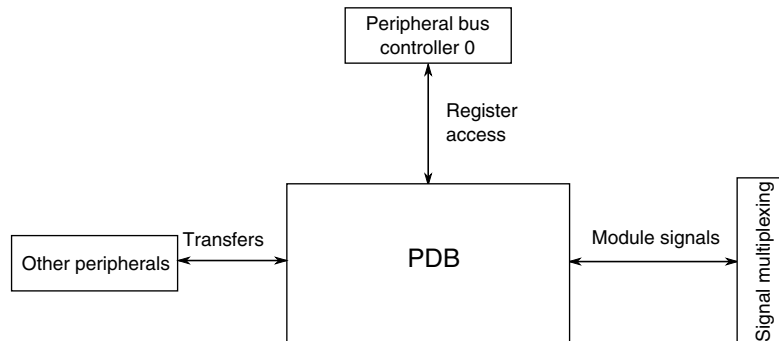
Figure 3-47. PDB configuration
