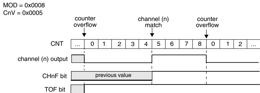
Figure 44-224. EPWM Signal with ELSnB:ELSnA = X:1
