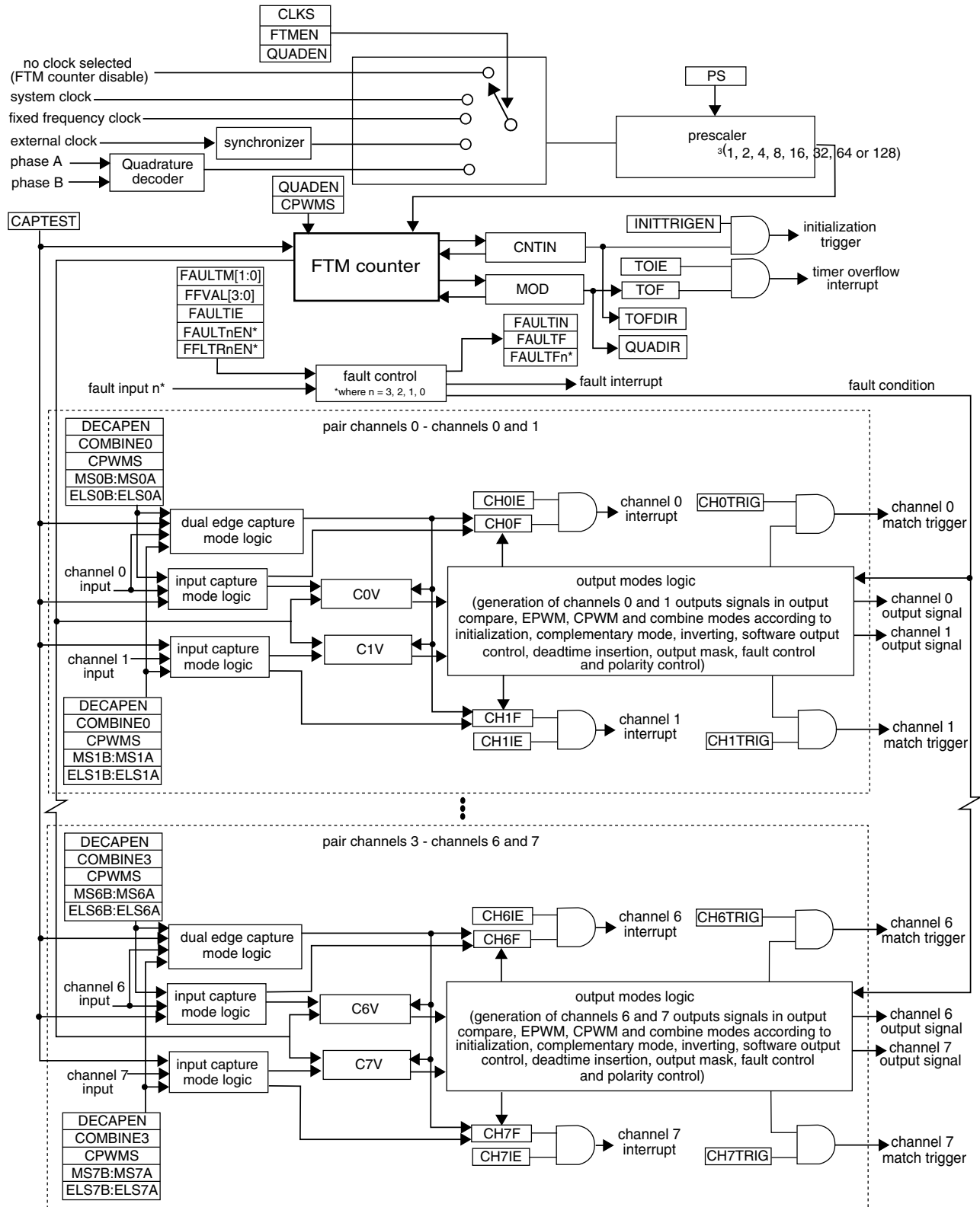
Figure 44-1. FTM Block Diagram
