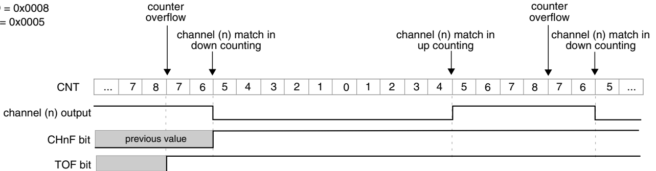
Figure 44-227. CPWM Signal with ELSnB:ELSnA = X:1
