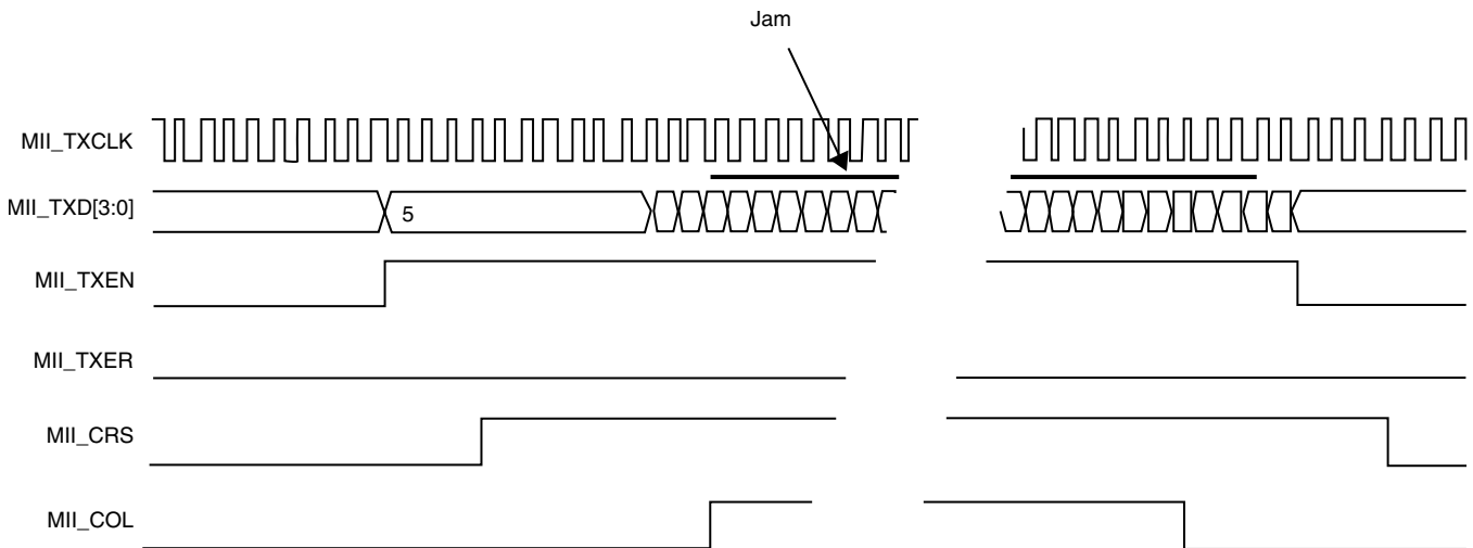
Figure 49-74. MII Transmit Operation — Transmission with Collision
