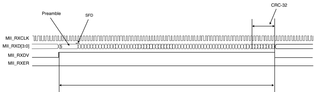
Figure 49-75. MII Receive Operation
