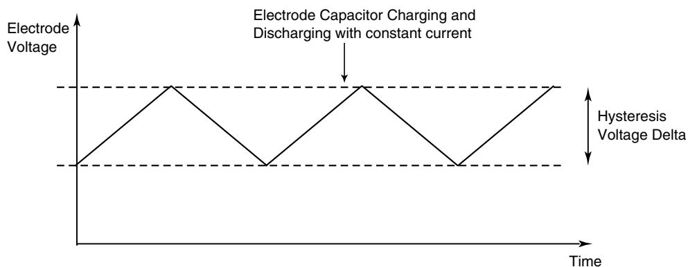
Figure 61-34. TSI electrode oscillator chart
