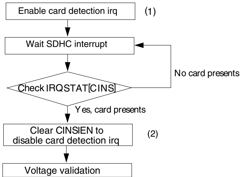
Figure 58-39. Flow diagram for card detection
