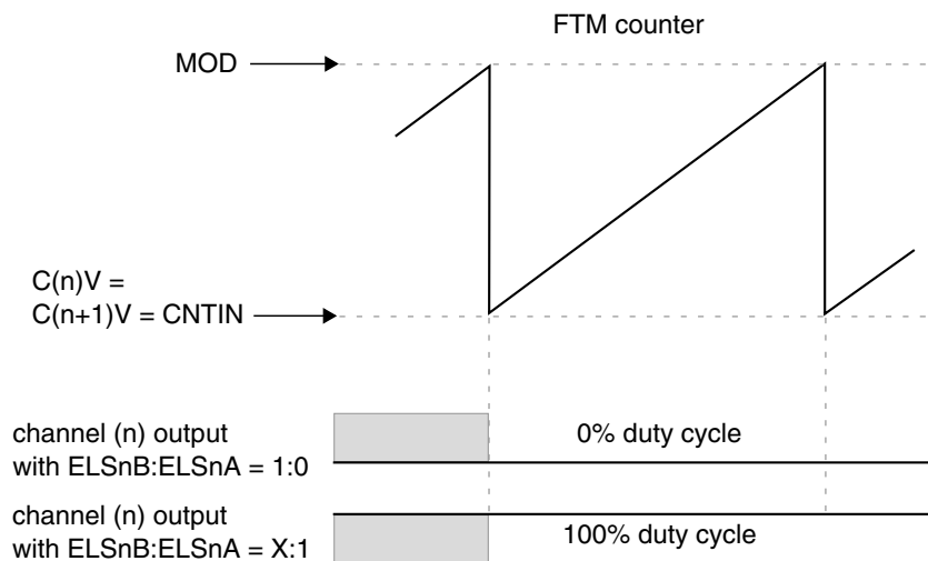
Figure 44-236. Channel (n) Output If (C(n)V = C(n+1)V = CNTIN)
