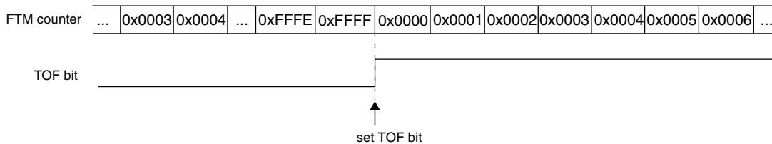
Figure 44-213. Example When the FTM Counter Is a Free Running
