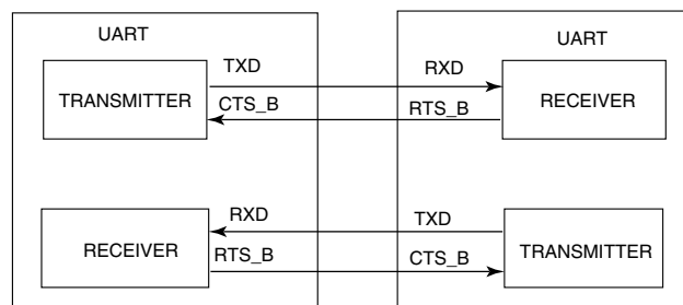
Figure 57-362. Ready-to-receive
