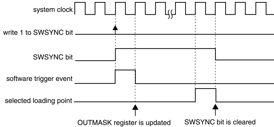
Figure 44-256. OUTMASK Synchronization with ( \text{SYNCMODE} = 0 ), ( \text{SYNCHOM} = 1 ), ( \text{PWMSYNC} = 0 ) and (Software Trigger Was Used)
