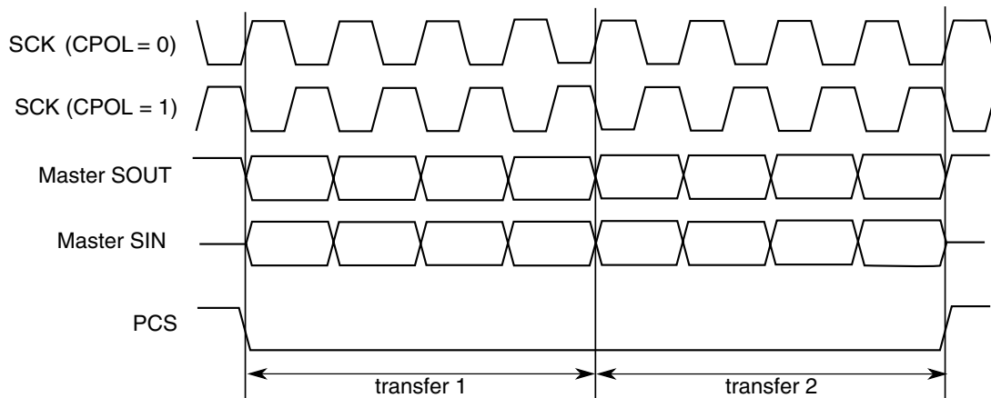
Figure 55-99. Continuous SCK Timing Diagram (CONT=1)
