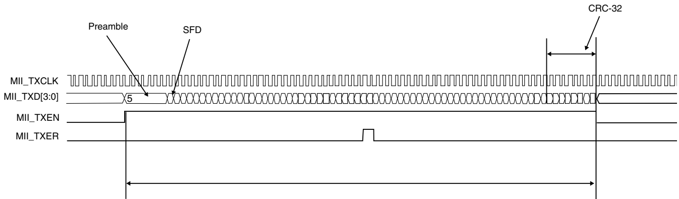
Figure 49-73. MII Transmit Operation — Errored Frame
