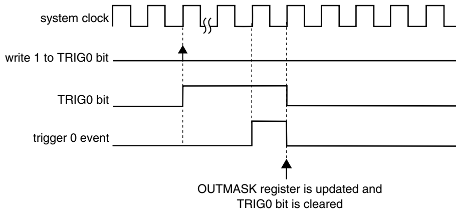
Figure 44-257. OUTMASK Synchronization with ( \text{SYNCMODE} = 0 ), ( \text{HWTRIGMODE} = 0 ), ( \text{SYNCHOM} = 1 ), ( \text{PWMSYNC} = 0 ), and (a Hardware Trigger Was Used)
