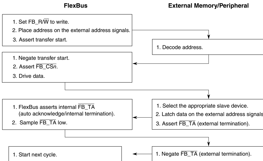
Figure 33-28. Write-Cycle Flowchart
