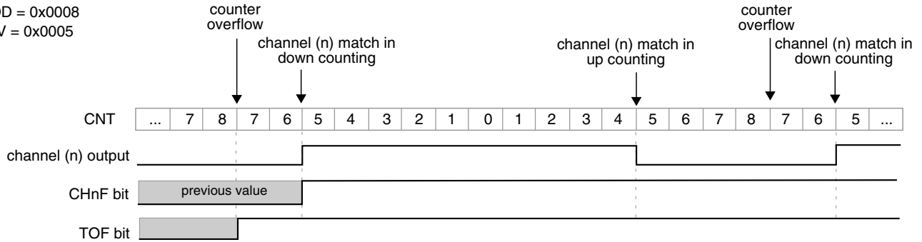
Figure 44-226. CPWM Signal with ELSnB:ELSnA = 1:0
