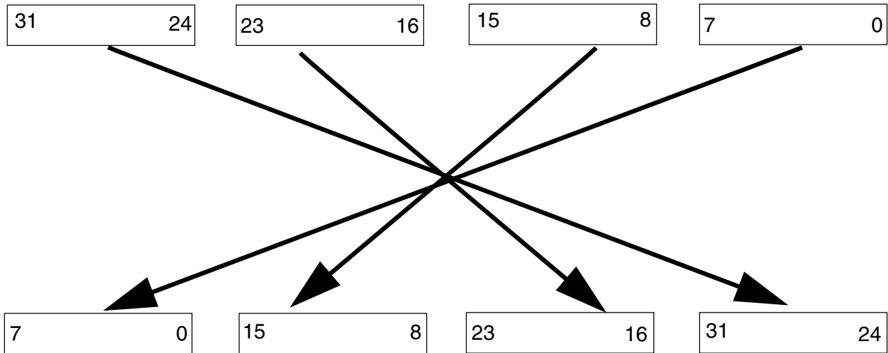
Figure 35-7. Transpose type 11
