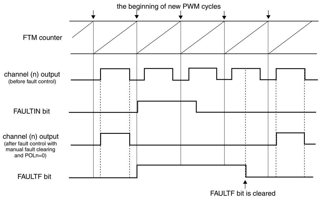
Figure 44-277. Fault Control with Manual Fault Clearing
