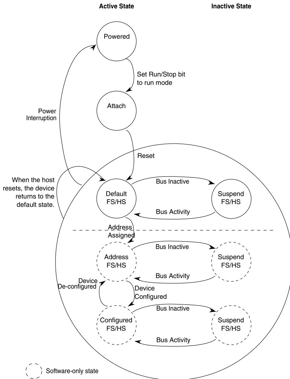
Figure 53-49. USB 2.0 Device States
