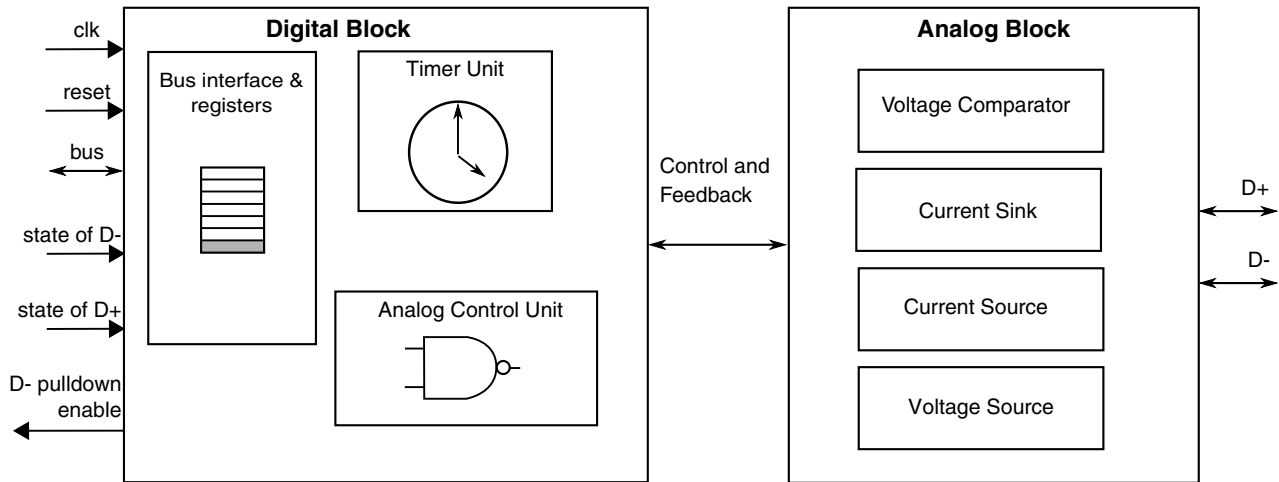
Figure 51-1. Block Diagram
