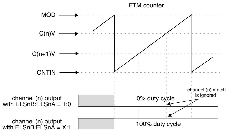
Figure 44-238. Channel (n) Output If (CNTIN < C(n)V < MOD) and (CNTIN < C(n+1)V < MOD) and (C(n)V > C(n+1)V)
