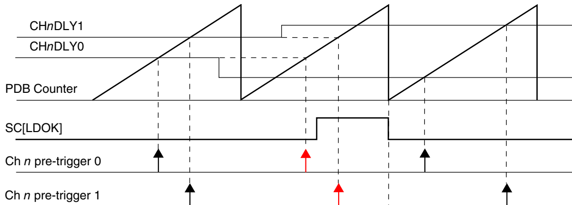
Figure 43-77. Registers Update with SC[LDMOD] = x1
