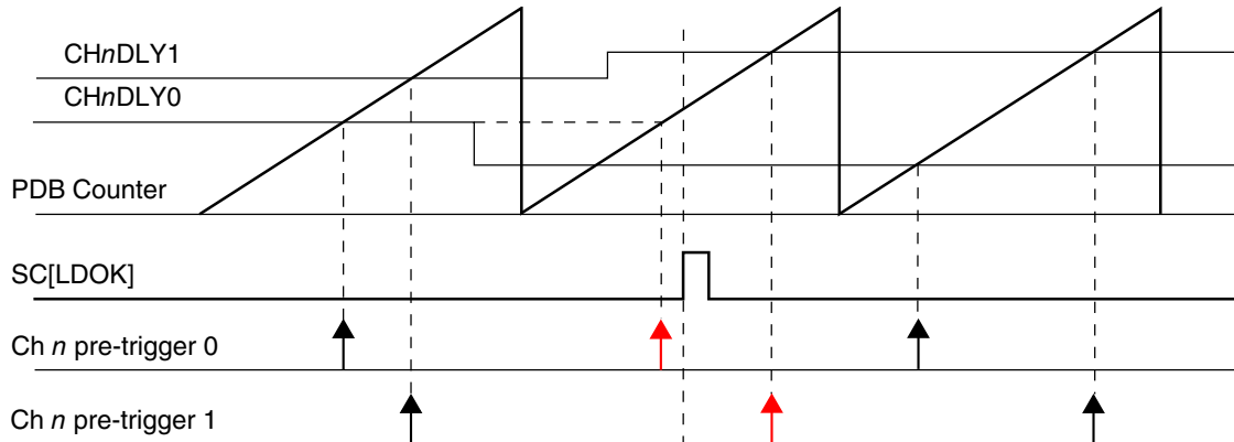
Figure 43-76. Registers Update with SC[LDMOD] = 00
