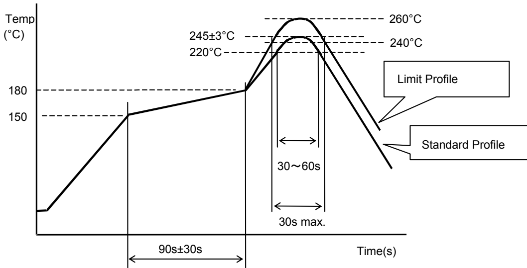
Soldering Profile for Lead Free solder (Sn-3.0Ag-0.5Cu solder )
