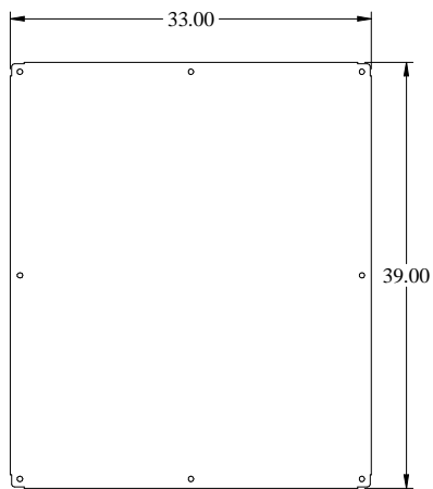
INNER PANEL
