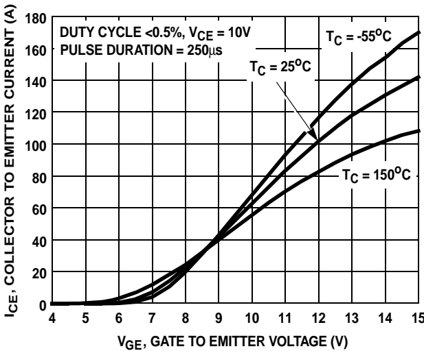
FIGURE 13. TRANSFER CHARACTERISTIC
