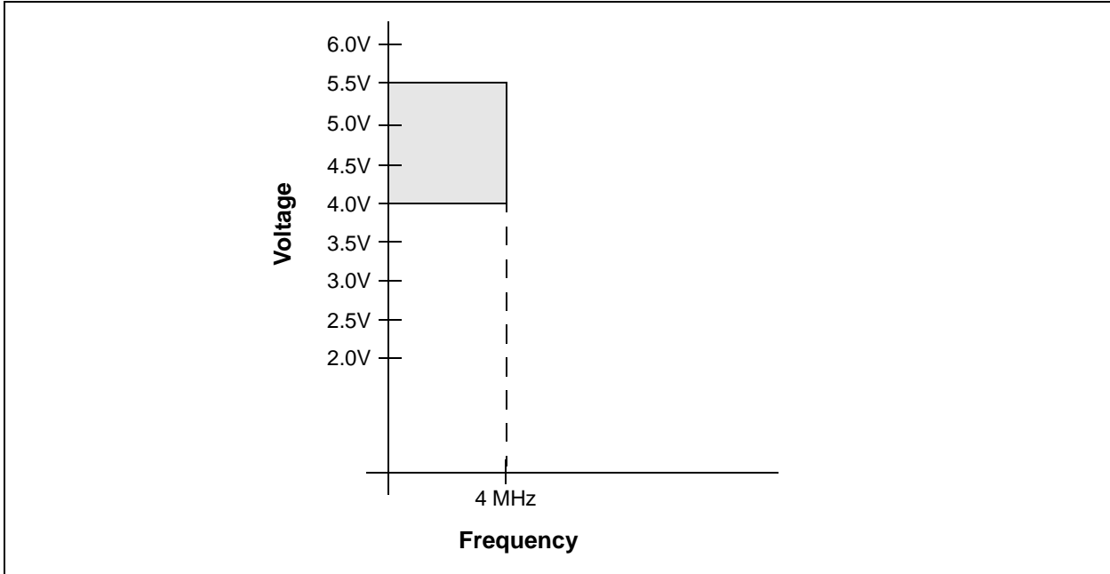
FIGURE 9-3: PIC16F84A-04 VOLTAGE FREQUENCY GRAPH
