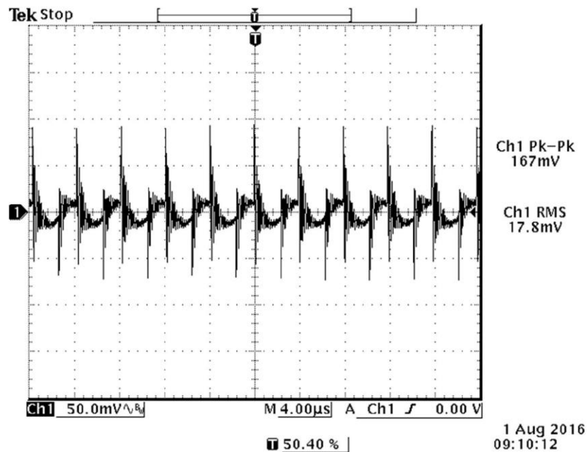
Figure 2. Ripple & noise 110 VDC input, 12 VDC/16.7 A output and T_a = 25^\circ\text{C} , and with a 1µF ceramic cap and 220µF electrolytic cap at output.
