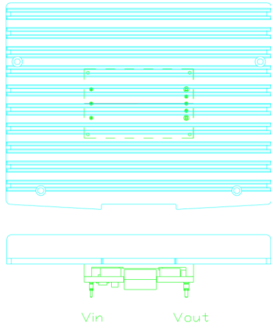
HSK Dimension:142x110x16mm (16 includes baseplate and ribs)
