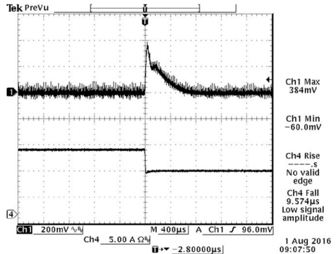
Figure 5. V_{out}=12V 75%-50% Load Transients at V_{in}=110V , T_a=25^\circ C
