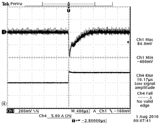
Figure 4. V_{out}=12V 50%-75% Load Transients at V_{in}=110V , T_a=25^\circ C
