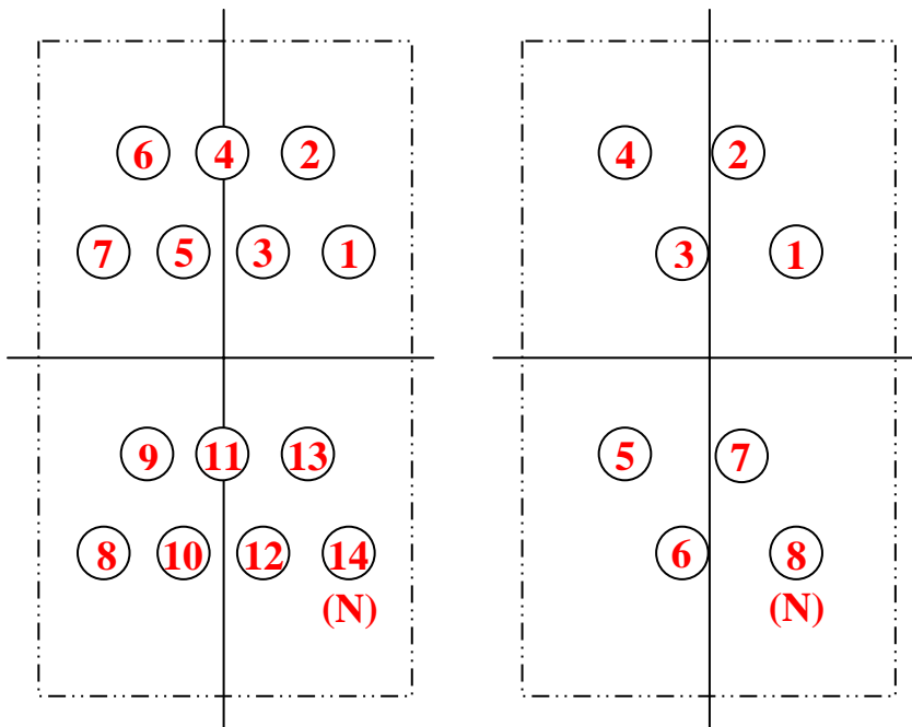
Odd # of Leads per Row
