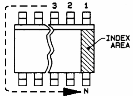
Device Top View Option B
