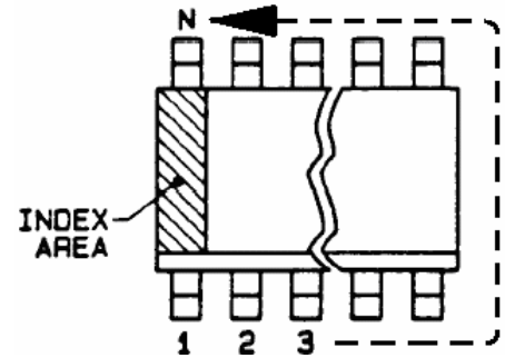
Device Top View Option A
