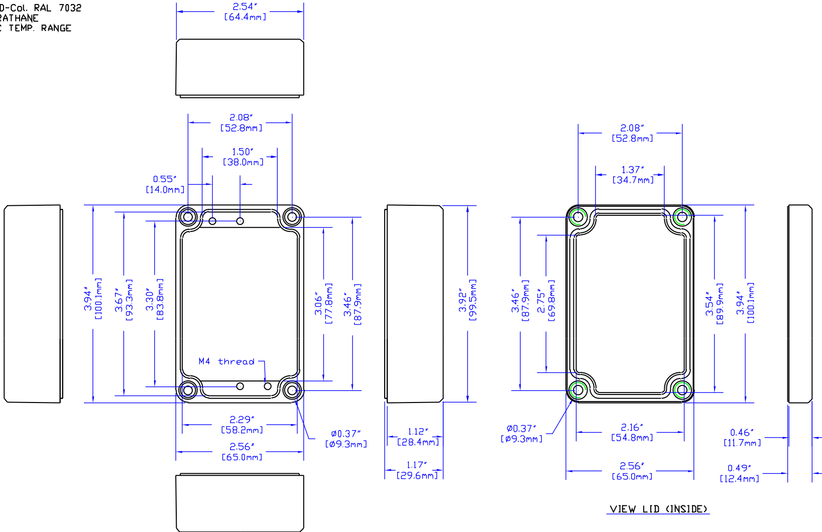
VIEW OF BOX (LID REMOVED)
