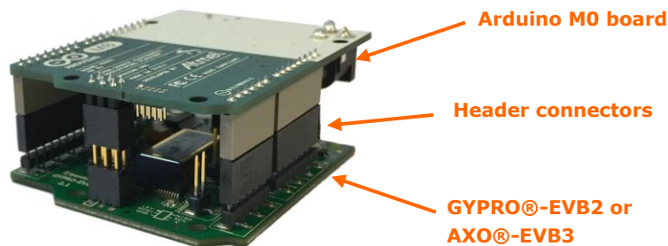
Figure 2: Correct position of the evaluation board
