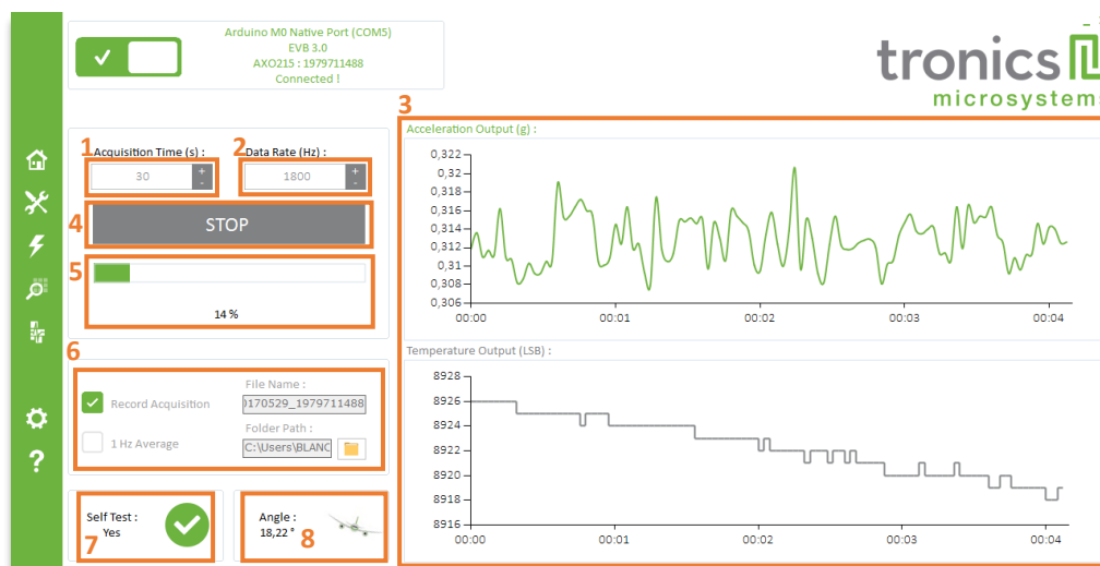
Figure 4: Tronics Evaluation Tool - "Reading Gypro" tab
