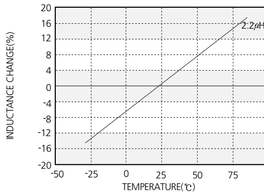
■ TEMPERATURE CHARACTERISTICS
