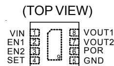
WDFN-8L 2x2
