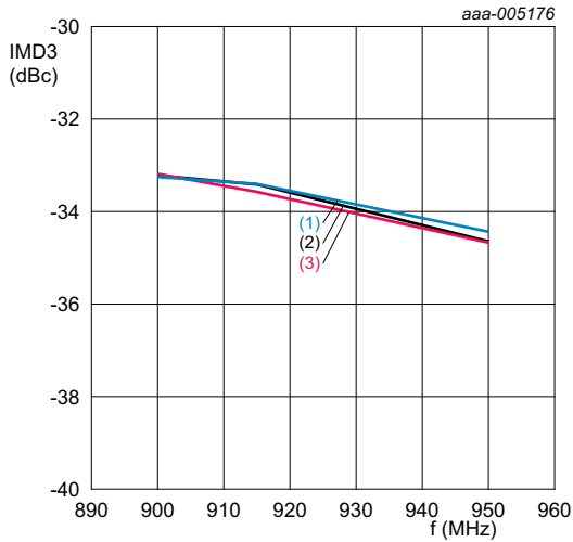
V_{SUP} = 3.6\text{ V}; I_{CC(tot)} = 70\text{ mA}; P_L = 15\text{ dBm} per tone; \Delta f = 1\text{ MHz}; matched for ISM-915. (1) T_{amb} = -40\text{ }^\circ\text{C} (2) T_{amb} = +25\text{ }^\circ\text{C} (3) T_{amb} = +85\text{ }^\circ\text{C}
