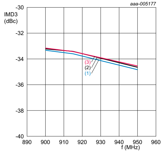
T_{amb} = 25\text{ }^\circ\text{C}; I_{CC(tot)} = 70\text{ mA}; P_L = 15\text{ dBm} per tone; \Delta f = 1\text{ MHz}; matched for ISM-915. (1) V_{SUP} = 3.3\text{ V} (2) V_{SUP} = 3.6\text{ V} (3) V_{SUP} = 3.9\text{ V}
