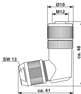
Dimensional drawing
