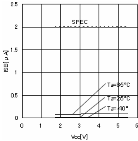
Figure 10. Standby current I_{SB}
