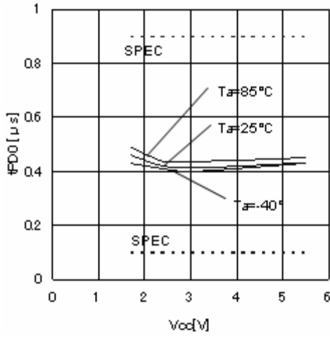
Figure 18. Output data delay time tPD0
