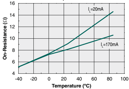
Typical On-Resistance vs. Temperature (I F =2mA)
