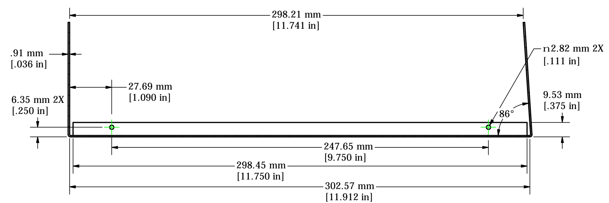
SECTION A-A SIDE SECTION VIEW OF EXPLODED ASSEMBLY
