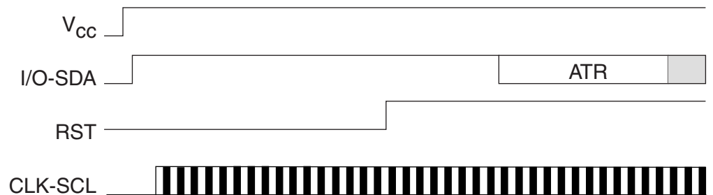
Figure 2. Asynchronous T = 0 Protocol (Gemplus Patent)
