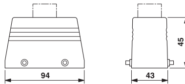
Dimensioned drawing
