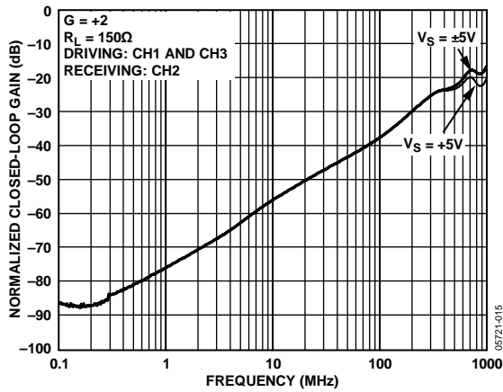
Figure 35. Worst-Case Crosstalk
