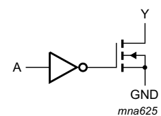
Fig 3. Logic diagram
