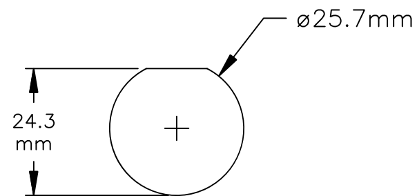
PANEL CUTOUT
