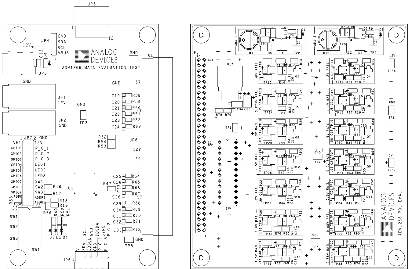
Figure 16. Top Silkscreen
