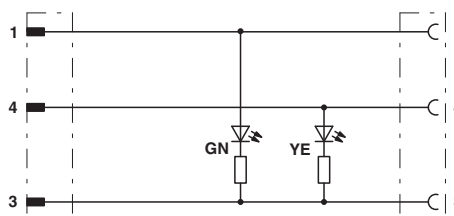
Contact assignment of M8 plugs / M12 sockets
