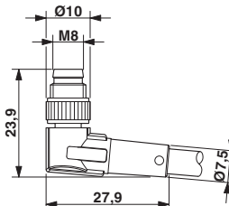
Dimensional drawing
