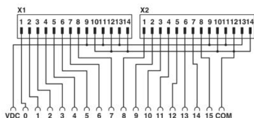
Connection scheme FLKM 14-PA-SLC500/OUT
