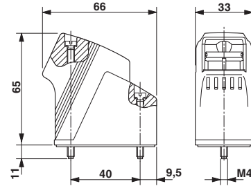
Dimensioned drawing
