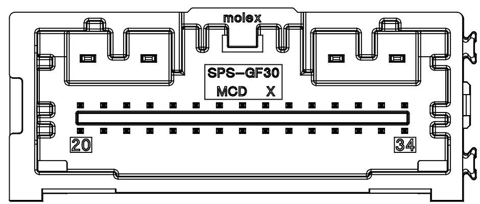
34WAY POLARIZATION OPTION 'B' P/N: 34958-0341
