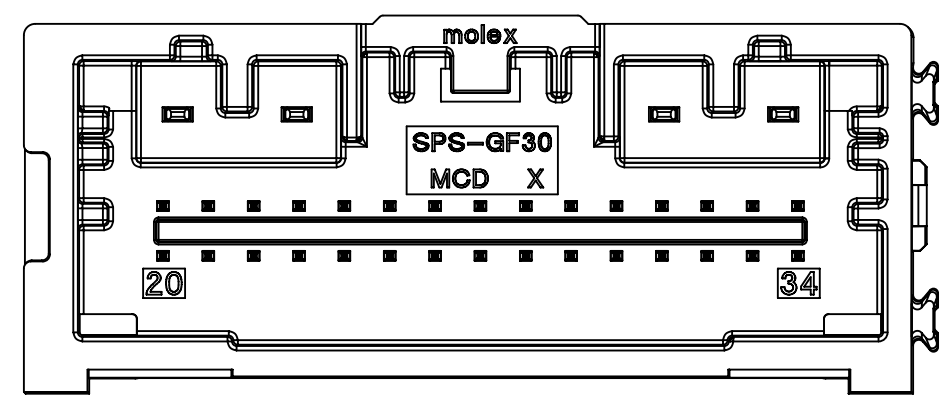
34WAY POLARIZATION OPTION 'A' P/N: 34958-0340
