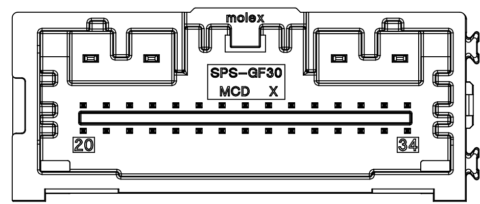
34WAY POLARIZATION OPTION 'C' P/N: 34958-0342
