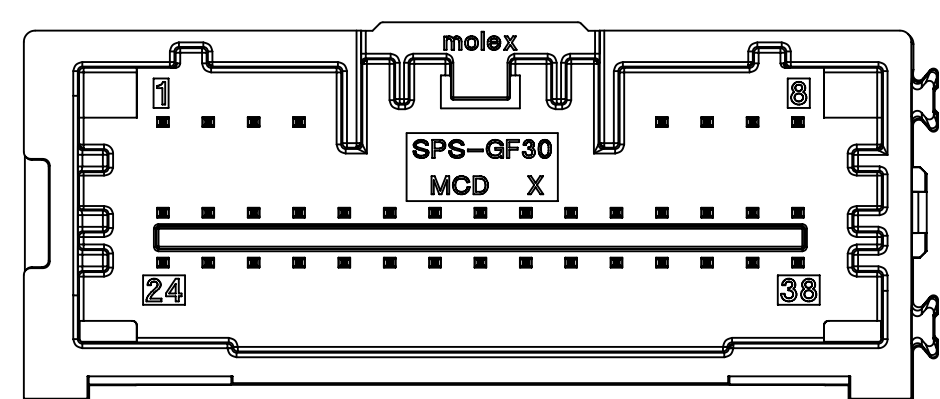
38WAY POLARIZATION OPTION 'C' P/N: 34958-0382
