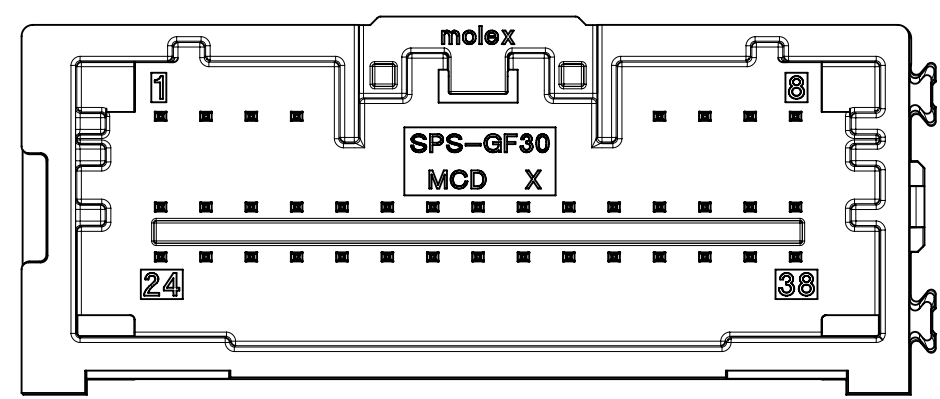
38WAY POLARIZATION UPDATED OPTION 'A' P/N: 34958-0383
