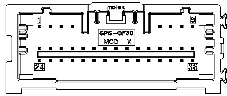
38WAY POLARIZATION OPTION 'A' P/N: 34958-0380
