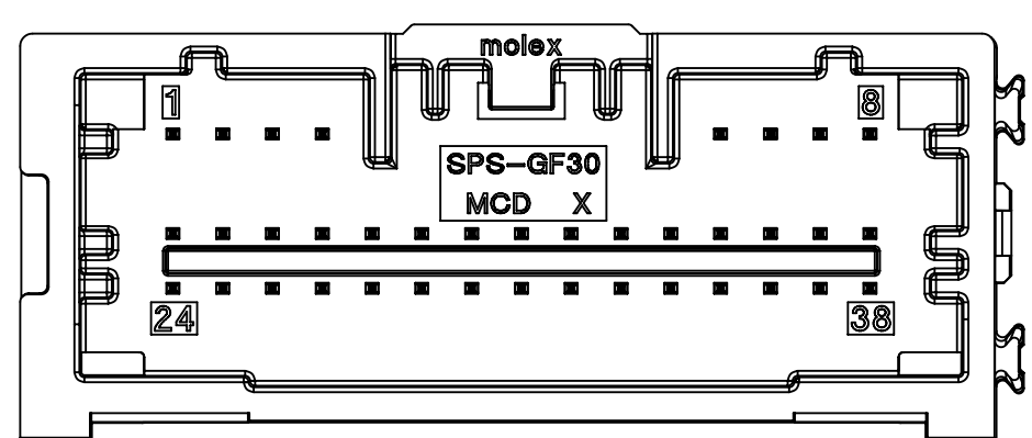
38WAY POLARIZATION OPTION 'B' P/N: 34958-0381
