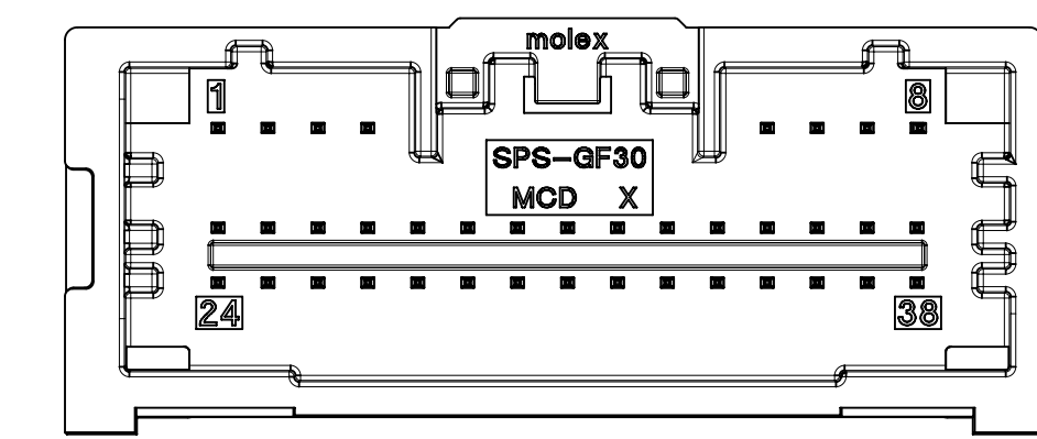
38WAY POLARIZATION UPDATED OPTION 'C' P/N: 34958-0385
