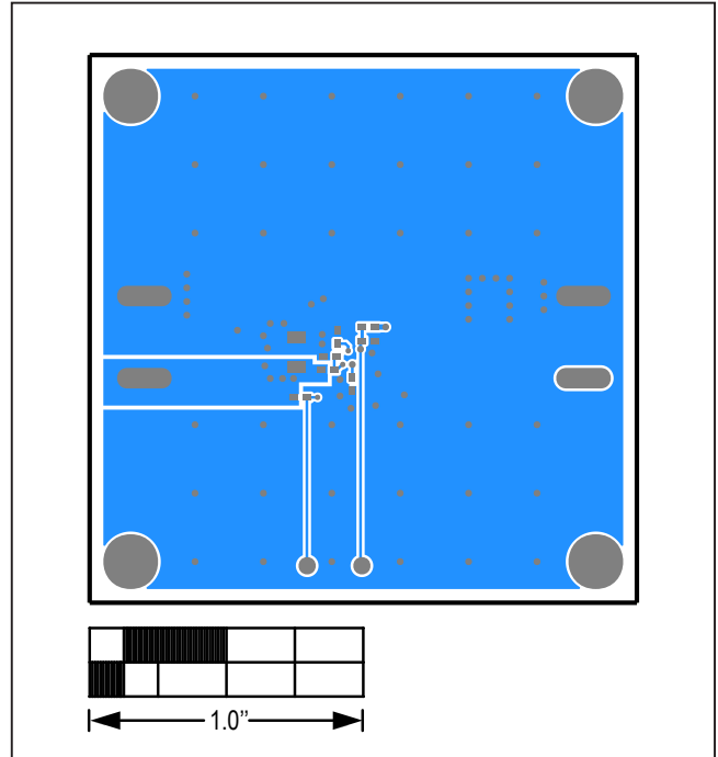
MAXM17532 EV Kit Bottom
