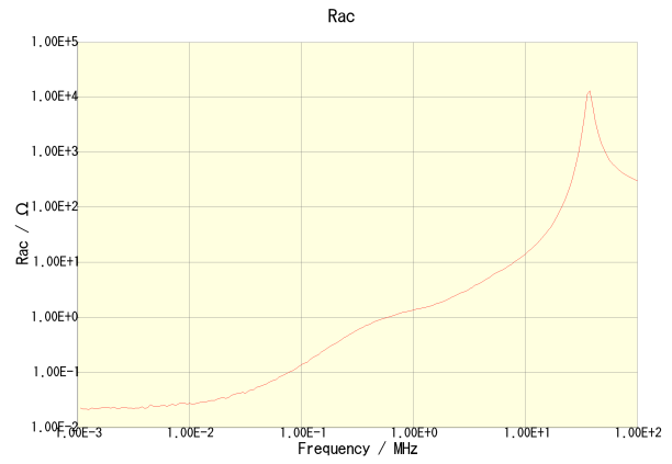
CLF7045T-100M-CA
