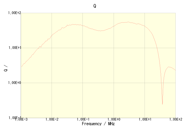
CLF7045T-100M-CA
