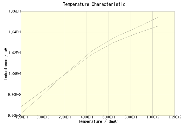
CLF7045T-100M-CA(DC = 0A)
