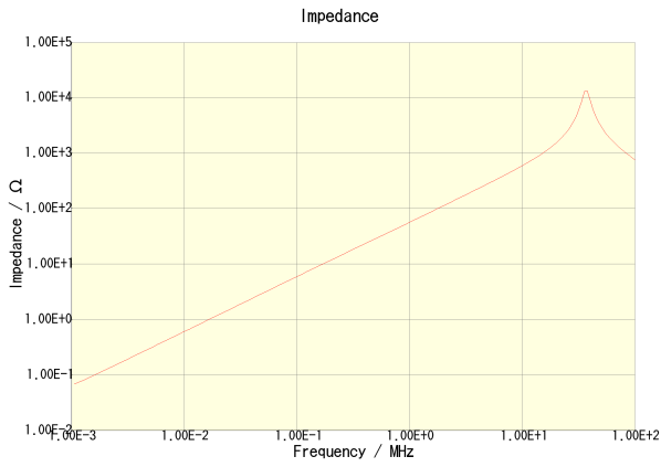
CLF7045T-100M-CA
