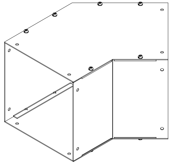
ISOMETRIC VIEW
