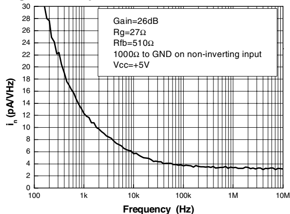
Figure 23. Input current noise
