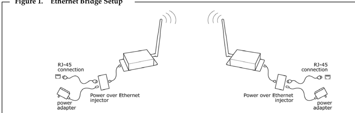
Figure 1. Ethernet Bridge Setup
