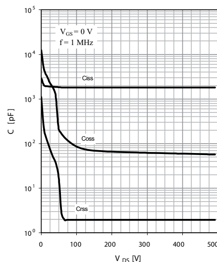
Fig. 9 Typ. capacitances
