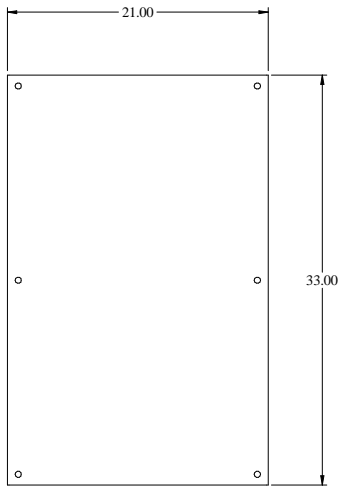
INNER PANEL
