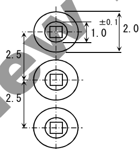
<3 lead pin type/2.5mm pitch>
