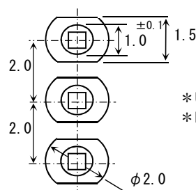
<3 lead pin type/2.0mm pitch>
